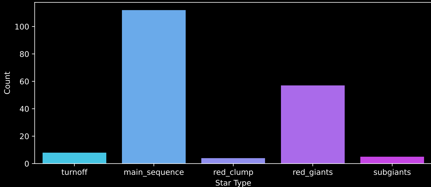
APOGEE DR17 Field: [K2_C18_215+36_btx] Count plot of Star Type
