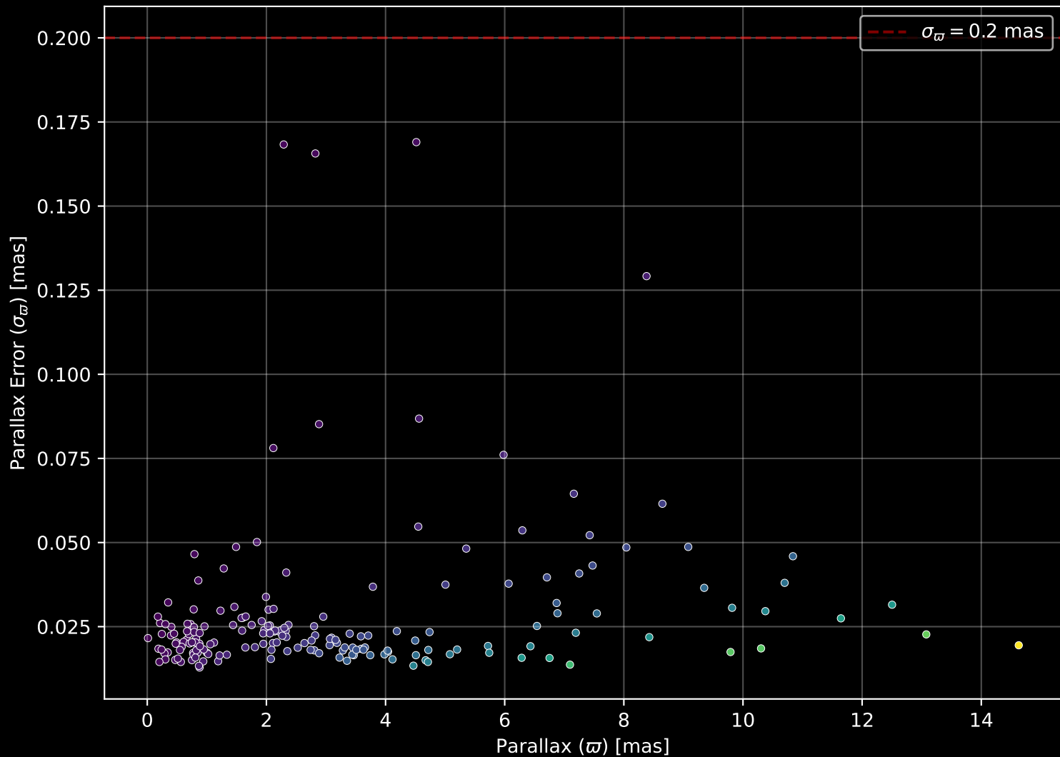
APOGEE DR17 Field: [K2_C18_215+36_btx] Parallax Quality (n= 186)
