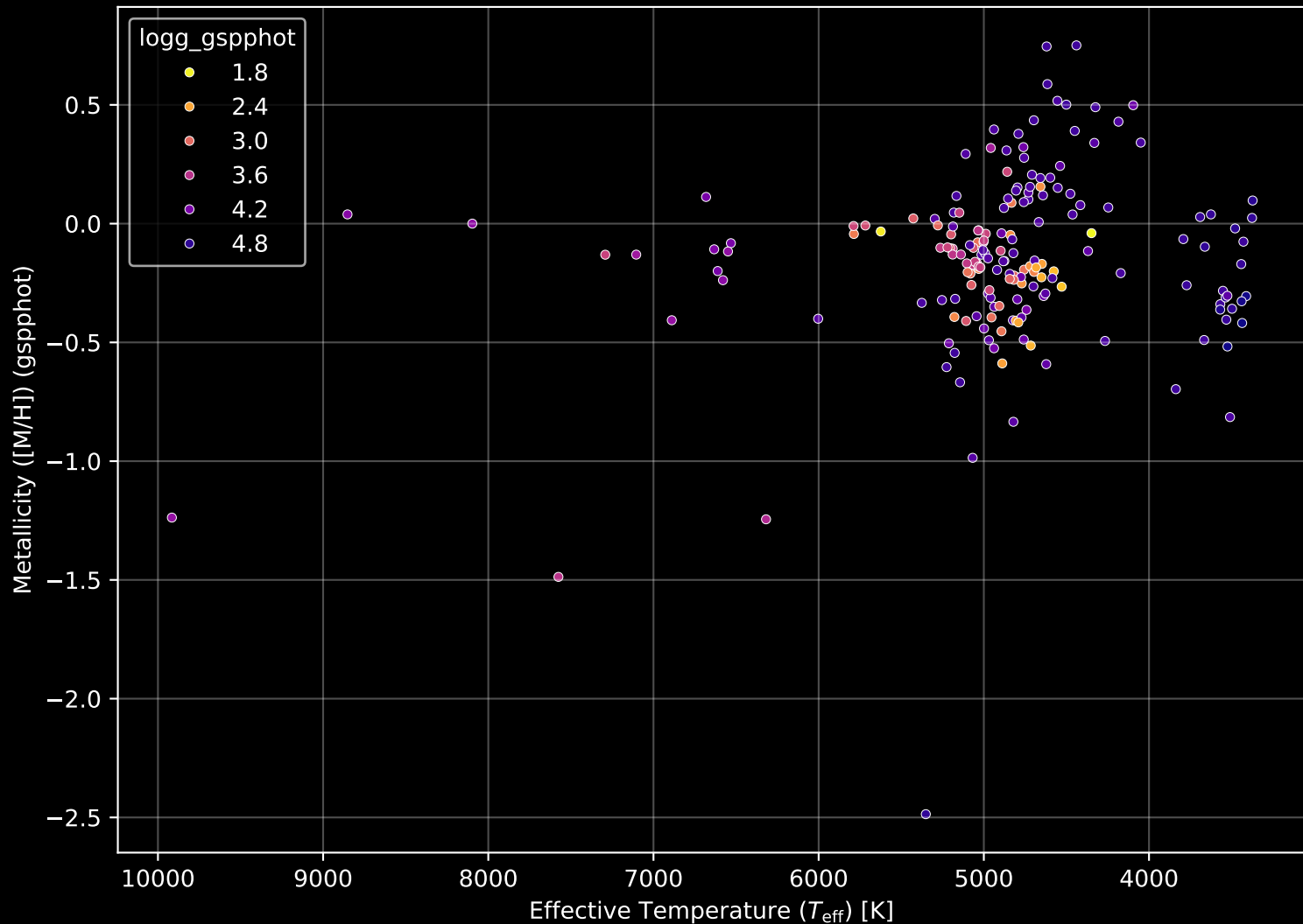
APOGEE DR17 Field: [K2_C18_215+36_btx] Stellar Population Parameters (n= 186)
