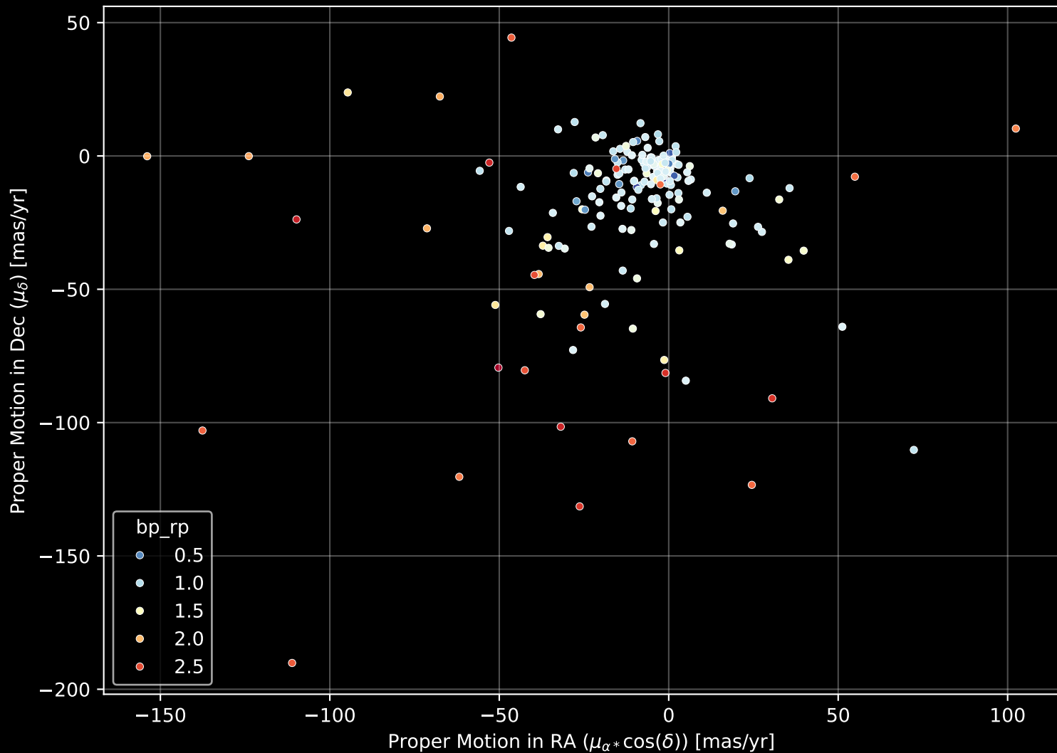
APOGEE DR17 Field: [K2_C18_215+36_btx] Proper Motion Diagram (n= 186)
