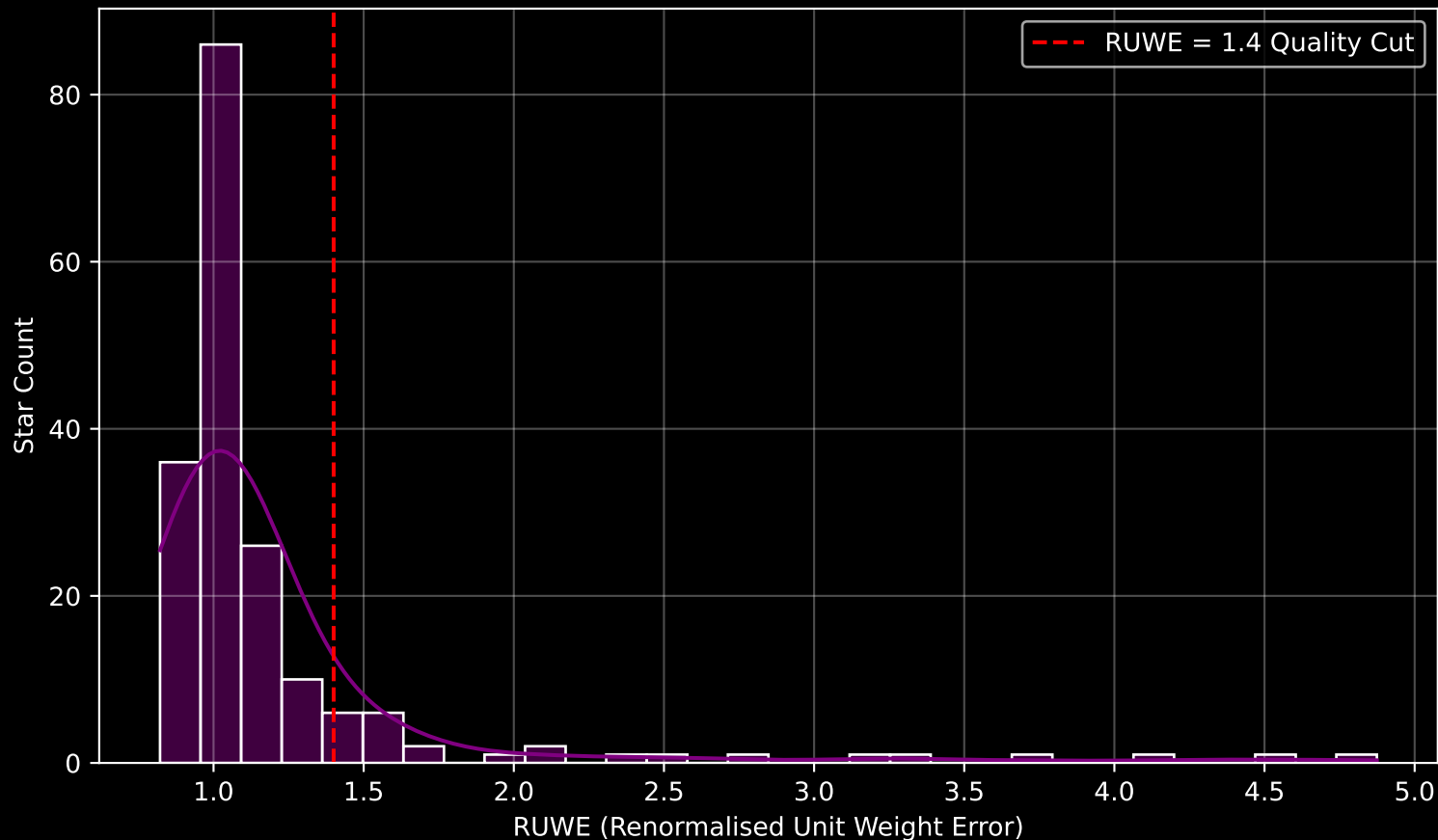
GAPOGEE DR17 Field [K2_C18_215+36_btx] RUWE Distribution (n= 184)
