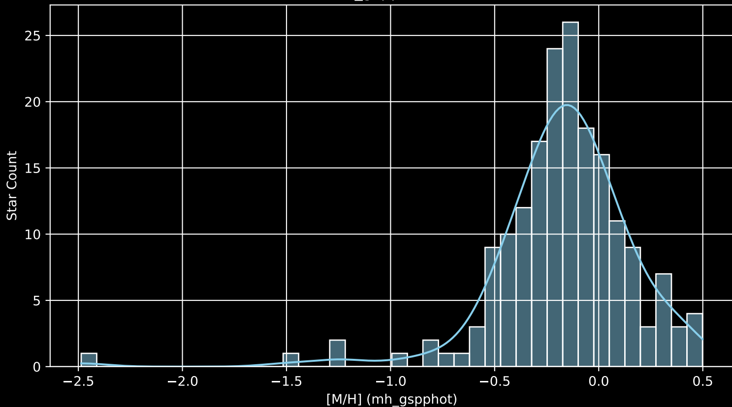
APOGEE DR17 Field: [K2_C18_215+36_btx [M/H] (mh_gspphot) (n= 181)
